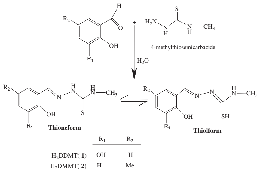
Scheme 1. Synthesis of H 2 DDMT (1) and H 2 DMMT (2).
